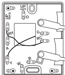
FIGURE 3 SOUS-SUPPORT
